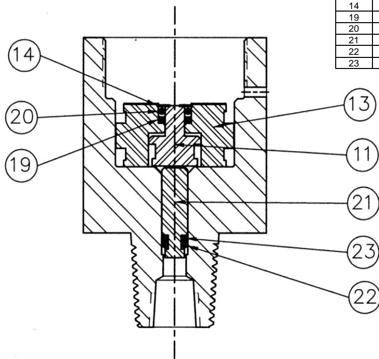
Figure 5: 1/4" Piston Arrangement Enlarged Detail Drawing For pressures from 1440 to 5900 PSI (99 to 407 bar)
