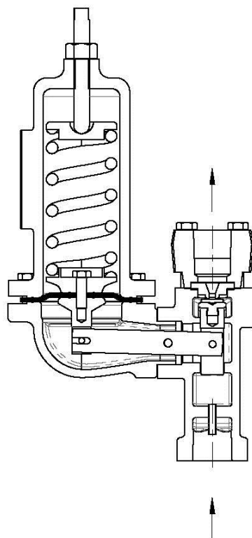
TYPE 630R RELIEF VAVLE OPERATIONAL SCHEMATIC
