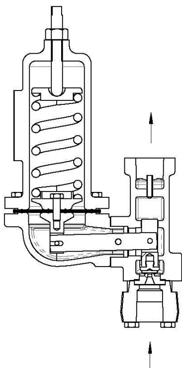
TYPE 630 REGULATOR OPERATIONAL SCHEMATIC
