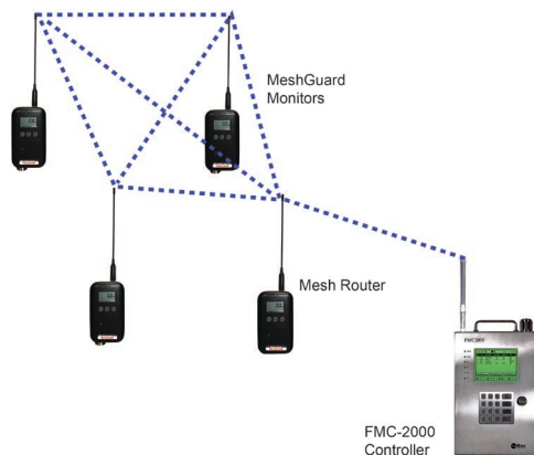
MeshGuard network with an FMC-2000 controller
