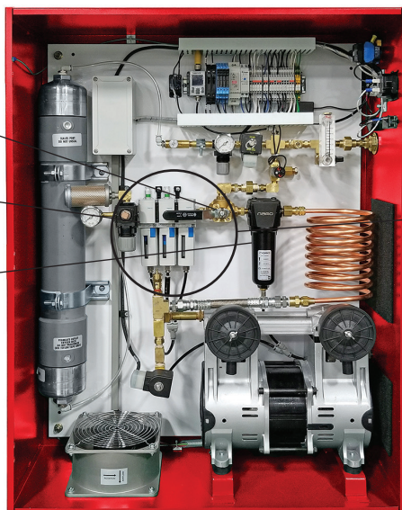
FIGURE 3 MODEL NG-1 100, NG-1 250 AND NG-1 500 WALL-MOUNTED NITROGEN GENERATOR FILTER CARTRIDGE REPLACEMENT
