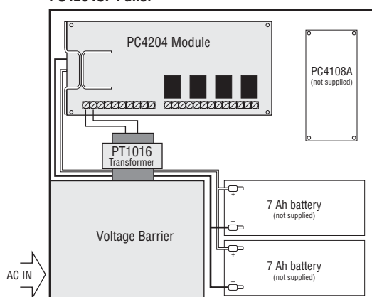
PC4204CF Panel
