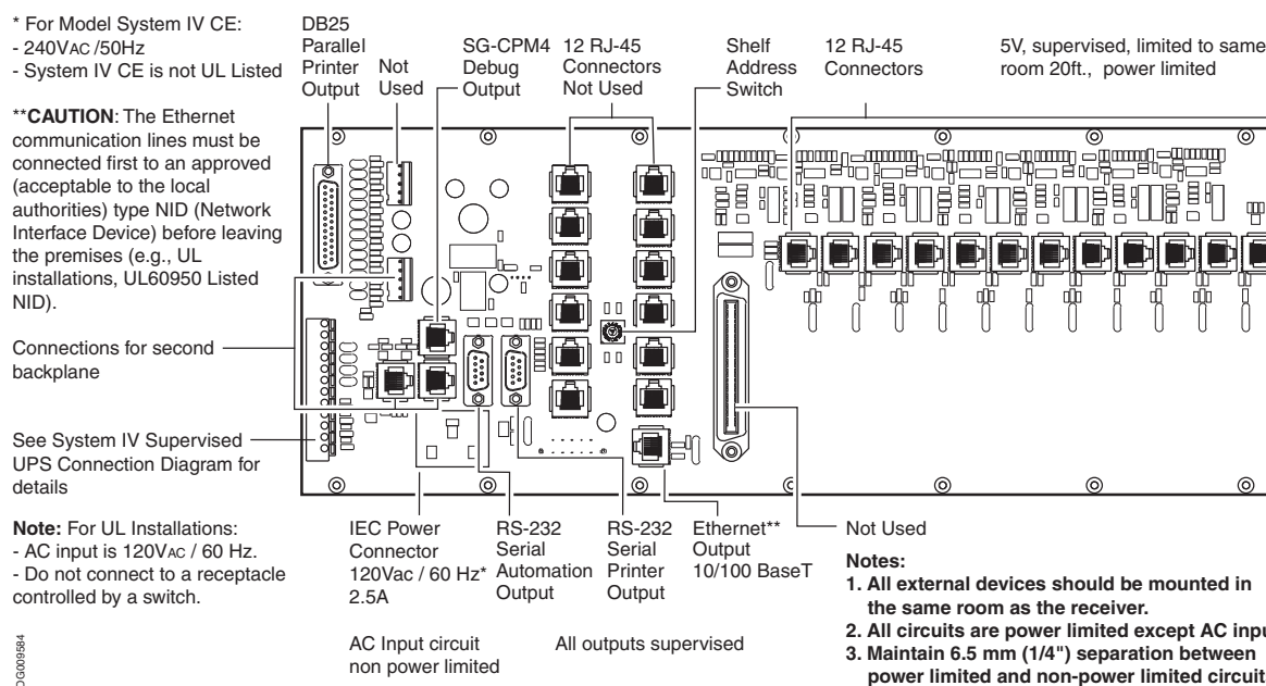
Figure 1-6 SG-System IV Wiring Diagram
