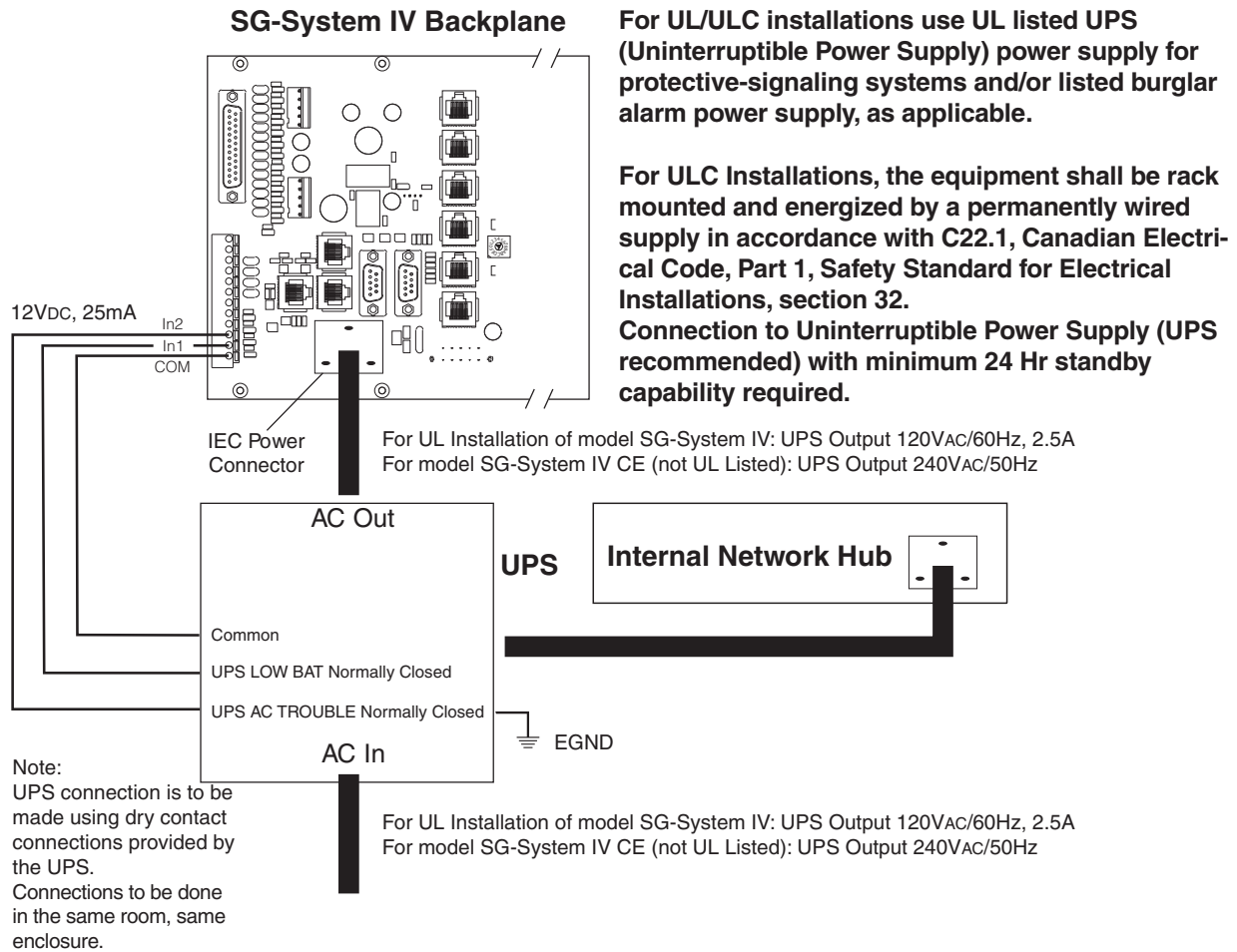
Figure 1-8 SG-System IV UPS Supervision Connection Diagram
