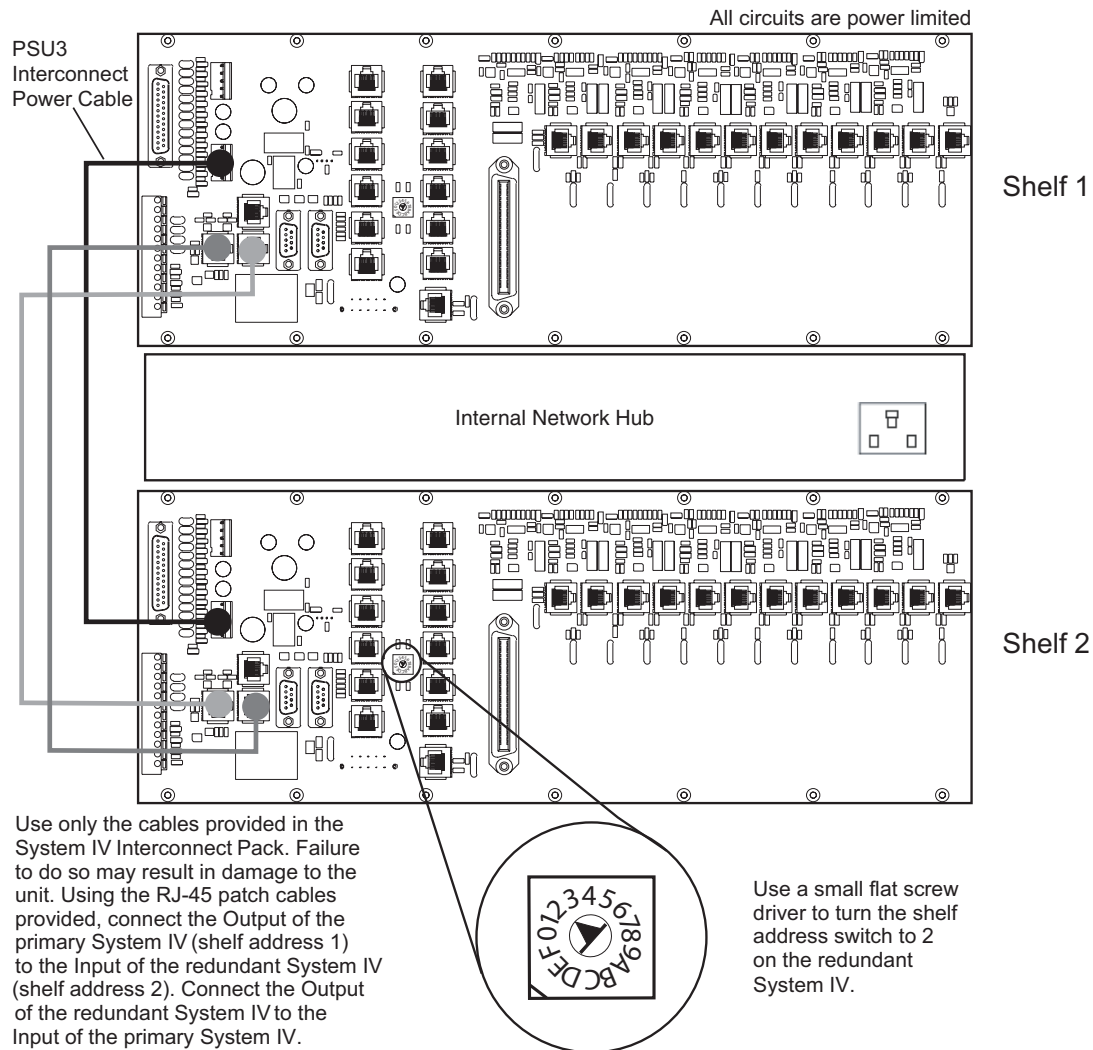
Figure 1-7 SG-System IV Redundancy Wiring Diagram
