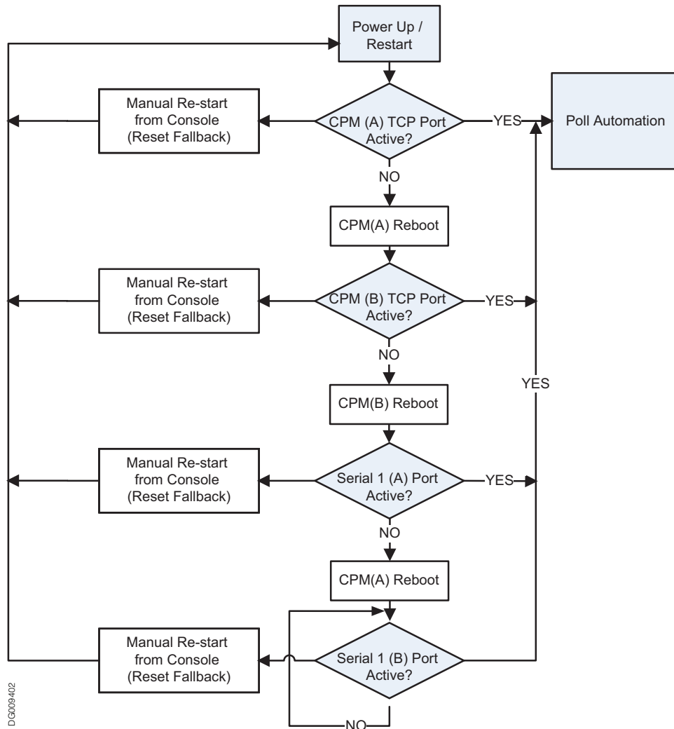
Flow Diagram for Automation IP Fallback Mode (3)
