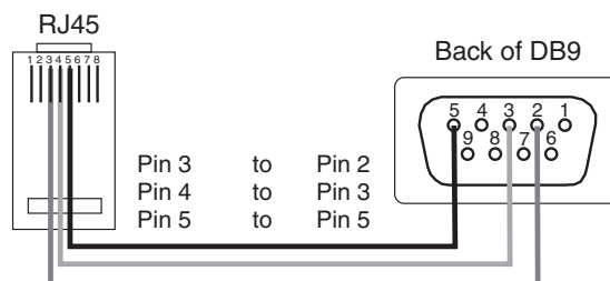
Figure 1-5 Figure 1-5 SG-DRL4-IP Debug Cable
