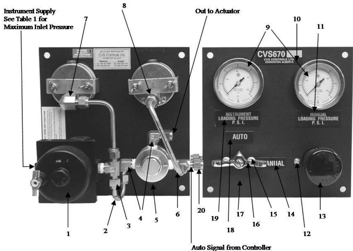
Figure 1: CVS Type 670GV Regulator Assembly
