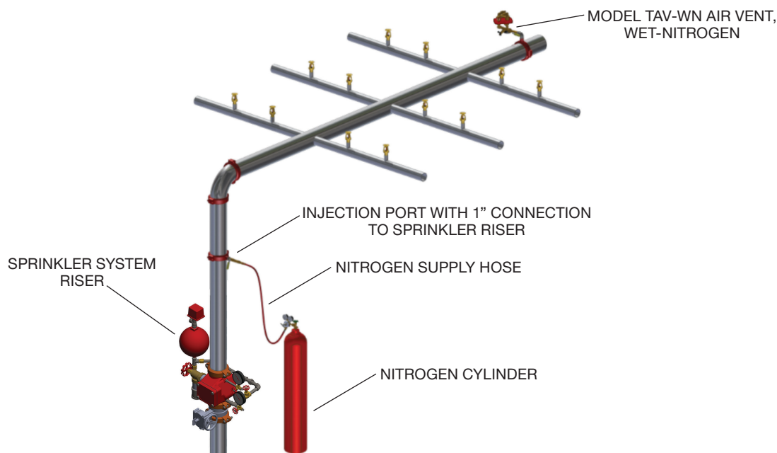
FIGURE 2 MODEL TNIP NITROGEN INJECTION PORT RISER INSTALLATION
