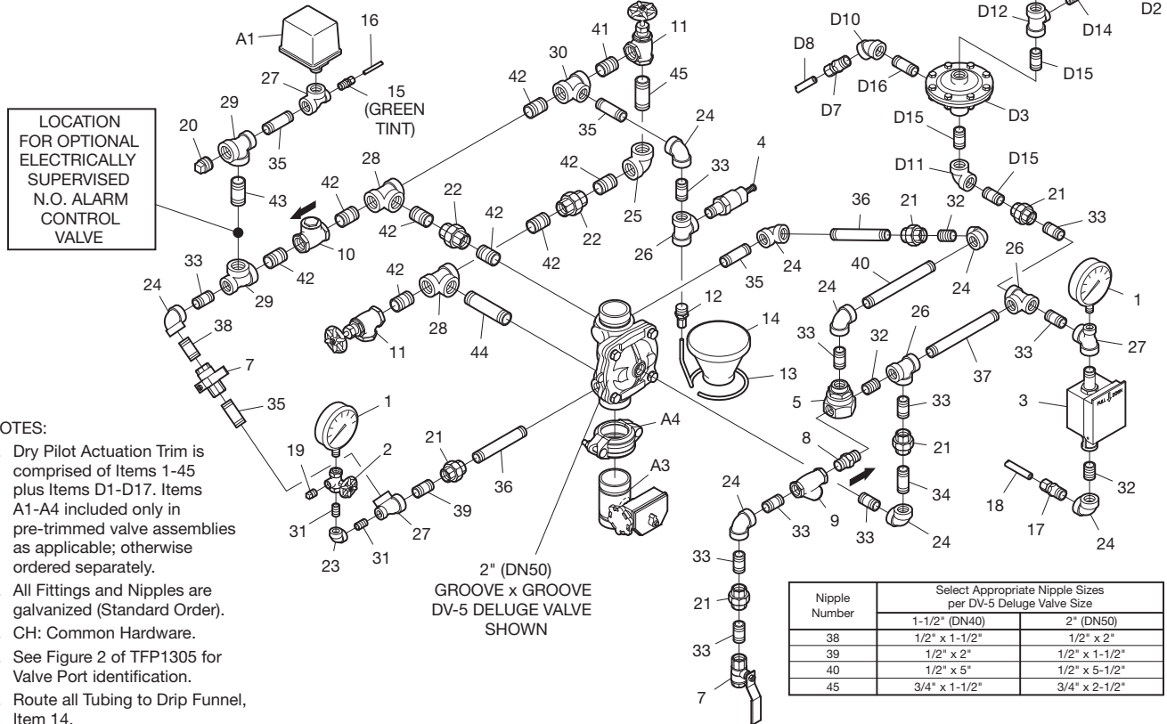
FIGURE 3A (1 OF 3) 1-1/2 AND 2 INCH (DN40 AND DN50) DV-5 DELUGE VALVES EXPLODED VIEW OF VERTICAL DRY PILOT ACTUATION TRIM
